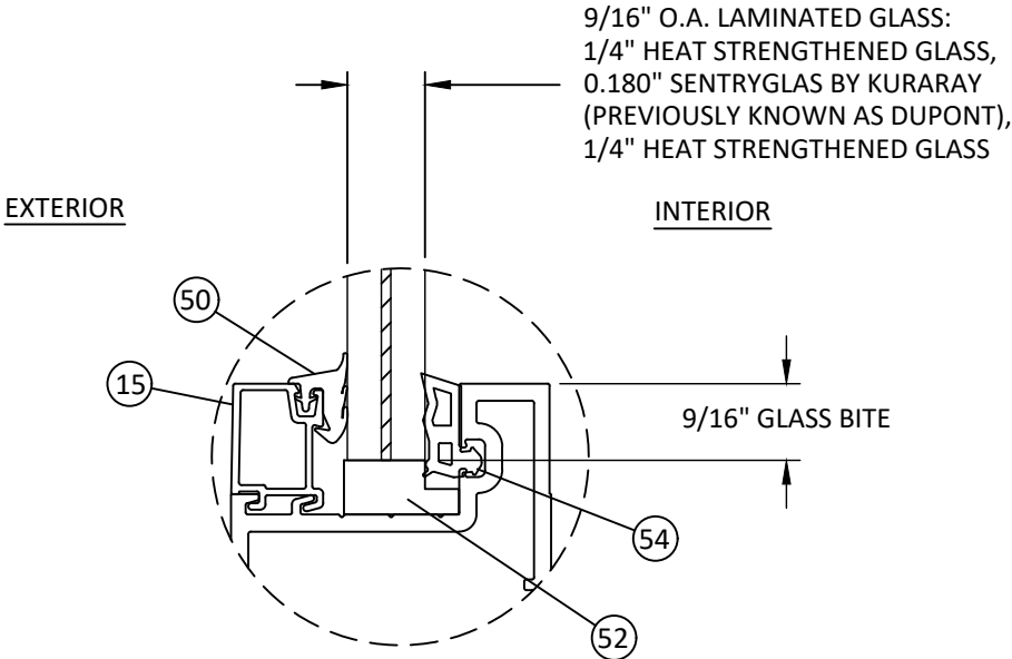
GLAZING DETAIL A (DRY GLAZED)
