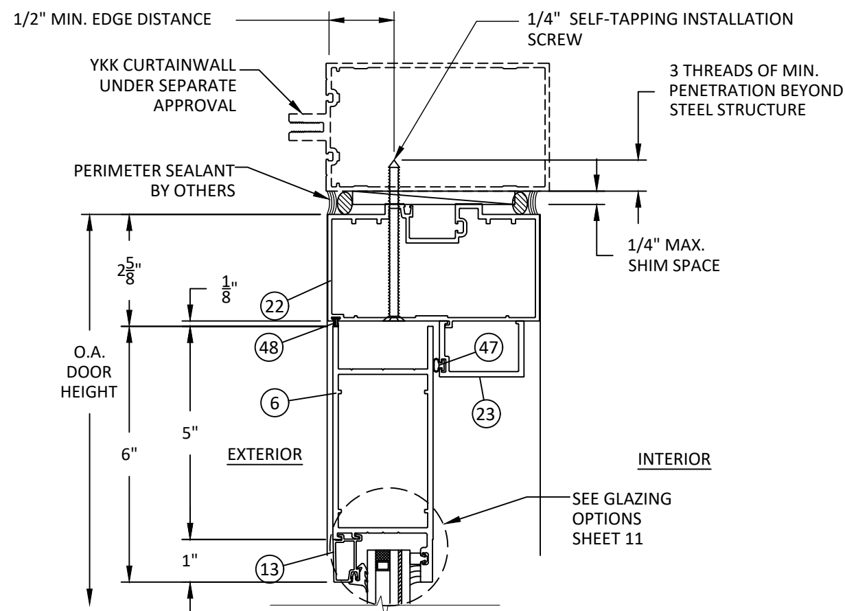
F 7 VERTICAL SECTION OHCC HEAD (OPTIONAL) TYP. CURTAINWALL MULLION
