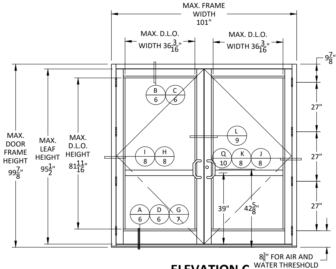
ELEVATION C CVR EXIT DEVICE STANDARD DOOR FRAME
