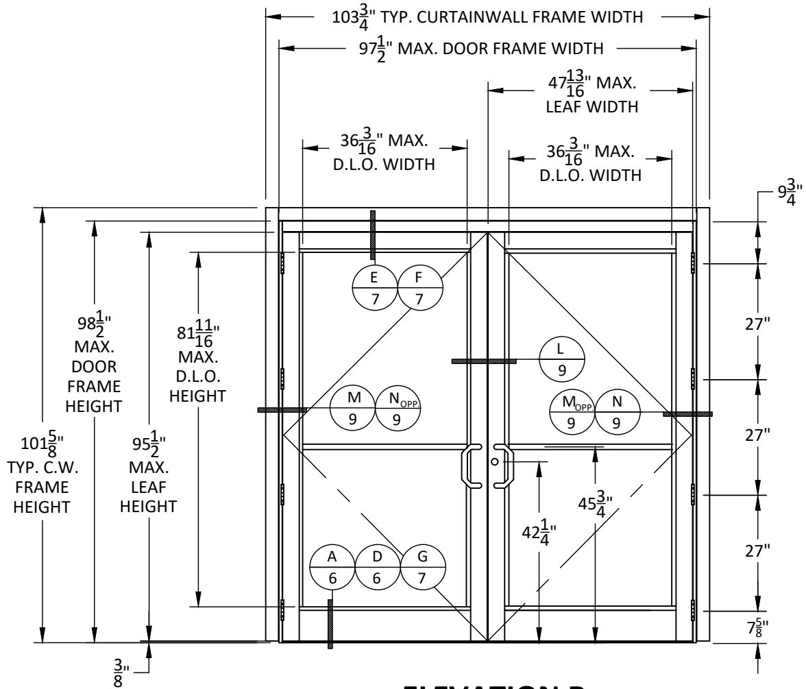
ELEVATION B STANDARD 5-POINT LOCK/CVR EXIT DEVICE STANDARD CURTAINWALL (C.W.) FRAMING
