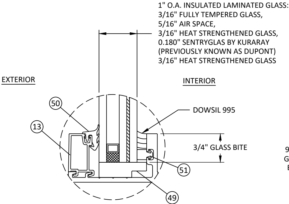
GLAZING DETAIL A1 (WET GLAZED)
