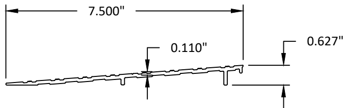
64 THRESHOLD RAMP INT./EXT. PIECE #1 6063-T5
