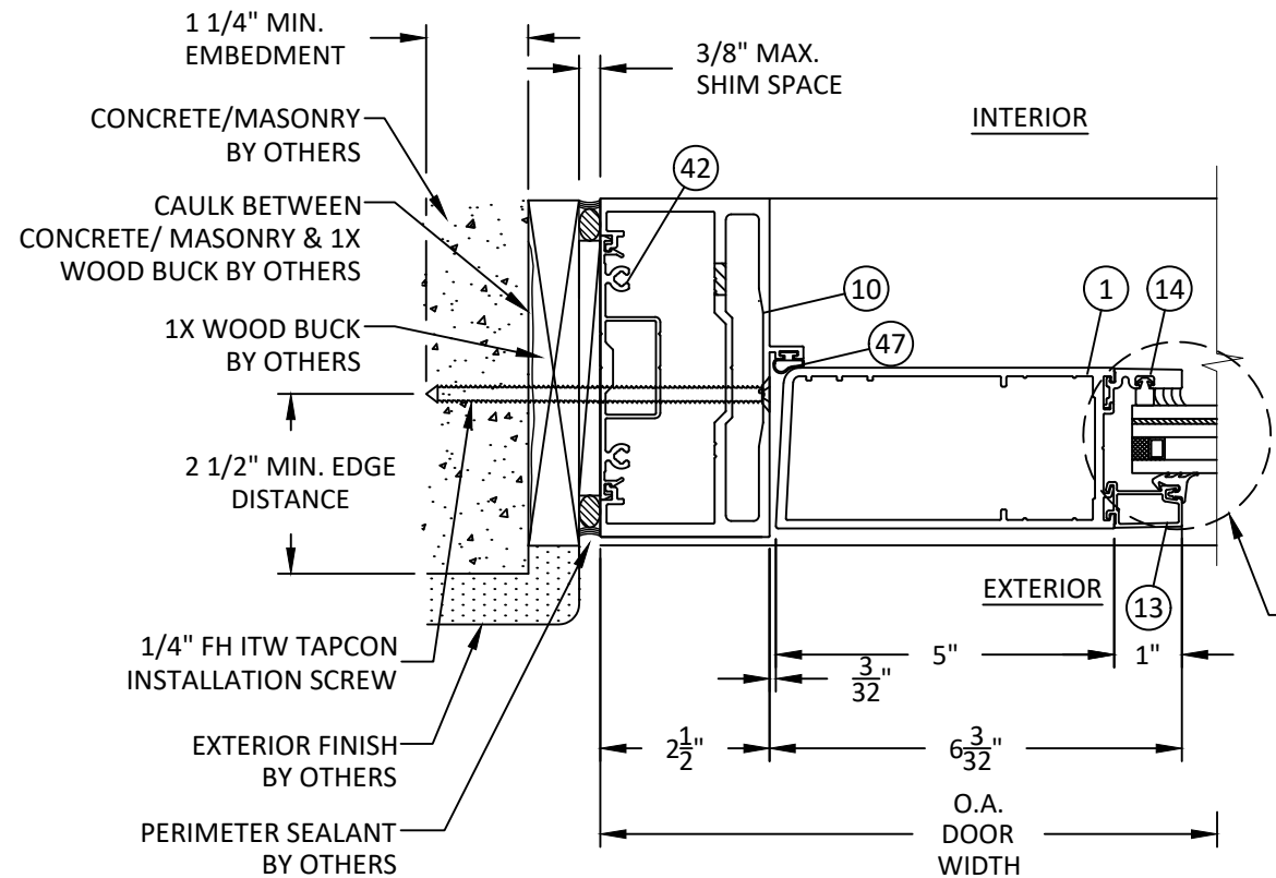
I HORIZONTAL SECTION 8 JAMB - CONCRETE/MASONRY
