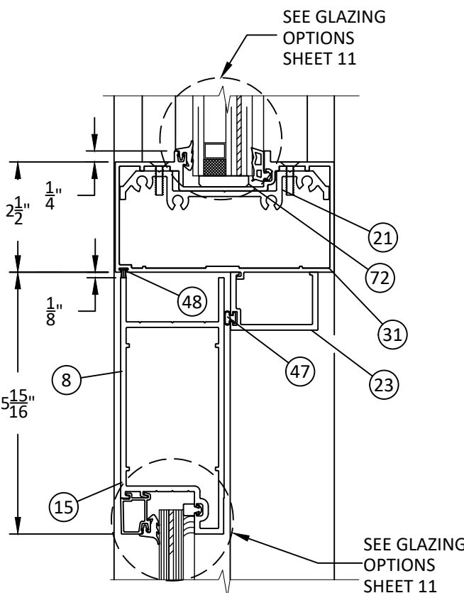
R 10 VERTICAL SECTION OHCC MULLION SEE SHEET 4 FOR DP LIMITATIONS
