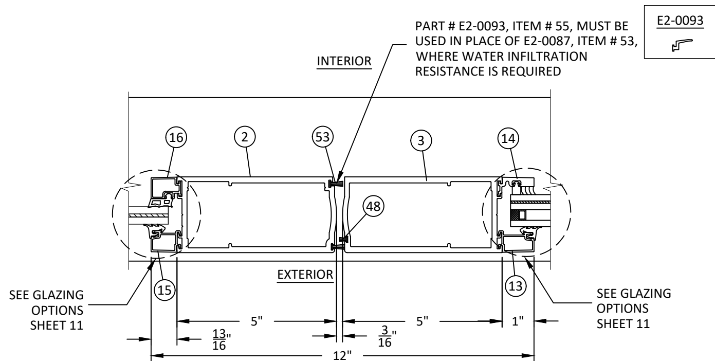
L9 HORIZONTAL SECTION MEETING STILES
