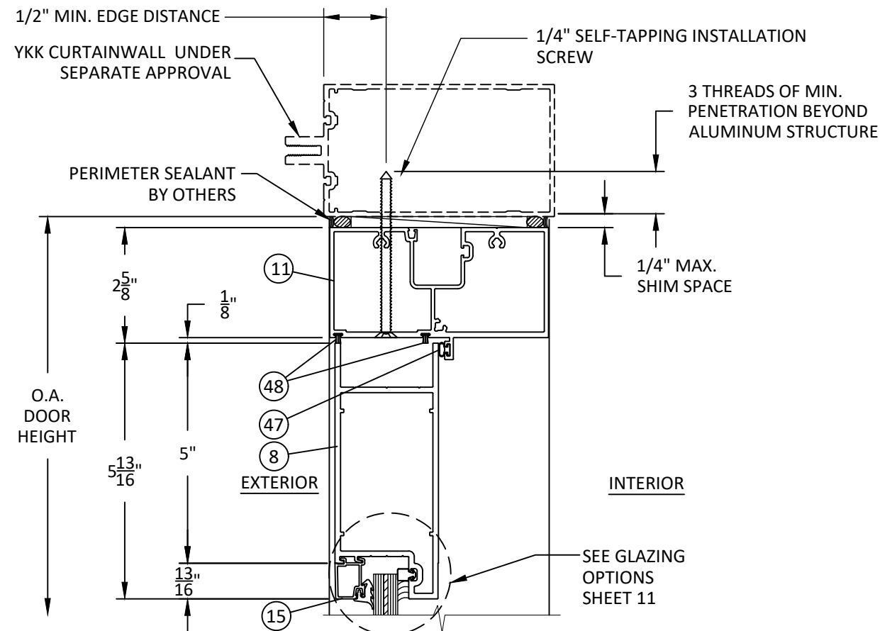
E 7 VERTICAL SECTION HEAD - TYP. CURTAINWALL MULLION
