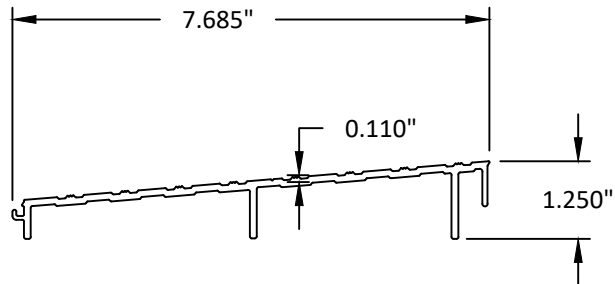
65 THRESHOLD RAMP INT./EXT. PIECE #2 6063-T5
