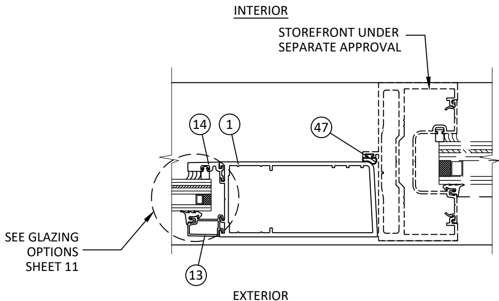
Q 10 HORIZONTAL SECTION VERTICAL MULLION STOREFRONT SYSTEM
