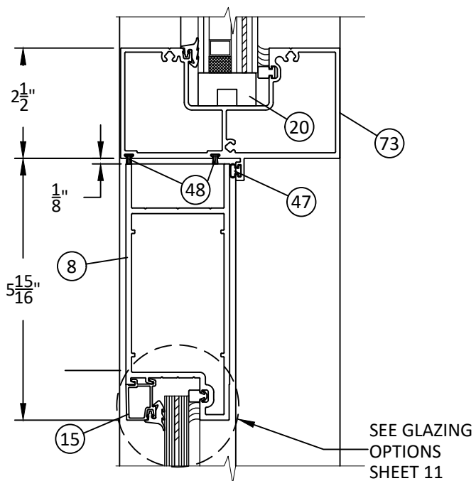
S 10 VERTICAL SECTION STANDARD TRANSOM MULLION SEE SHEET 4 FOR DP LIMITATIONS
