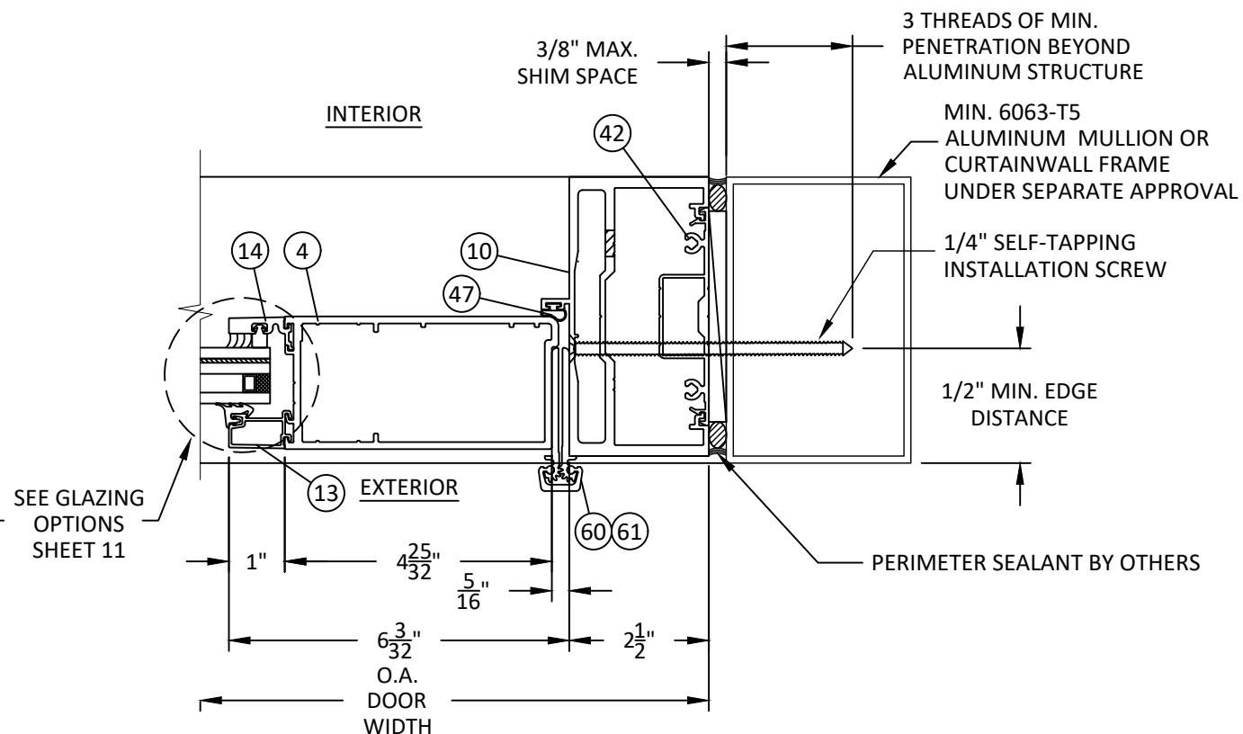
K HORIZONTAL SECTION 8 JAMB - ALUMINUM STUD CONTINUOUS HINGE
