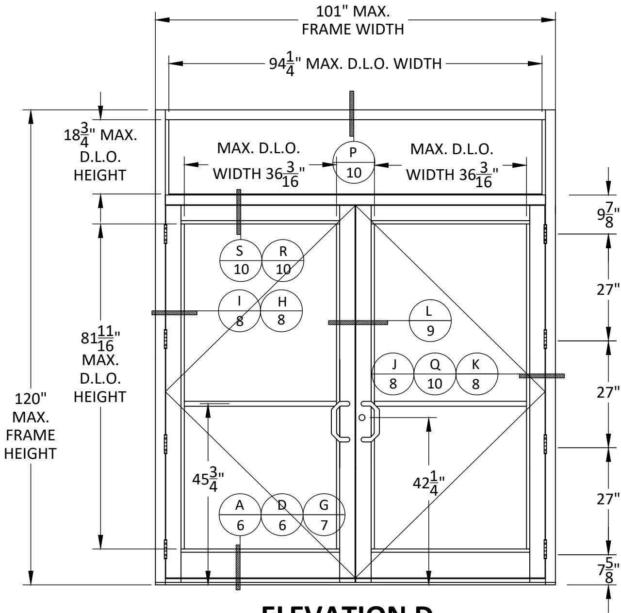
ELEVATION D DOUBLE DOOR WITH TRANSOM
