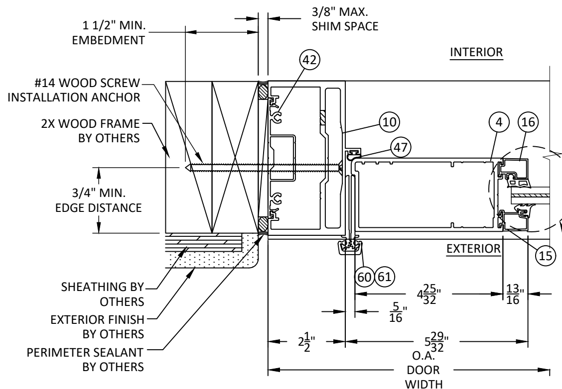
H HORIZONTAL SECTION 8 JAMB - 2XWOOD FRAME CONTINUOUS HINGE
