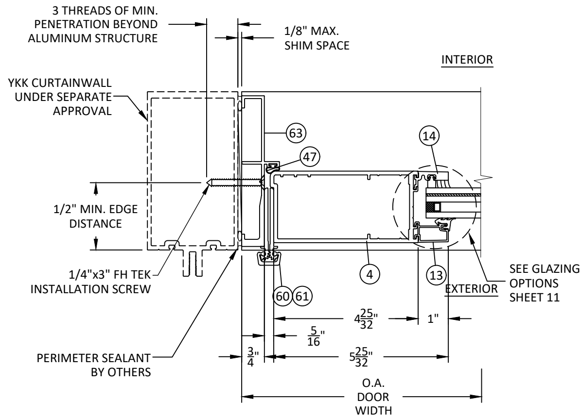
M9 HORIZONTAL SECTION JAMB - TYP. CURTAINWALL MULLION CONTINUOUS HINGE
